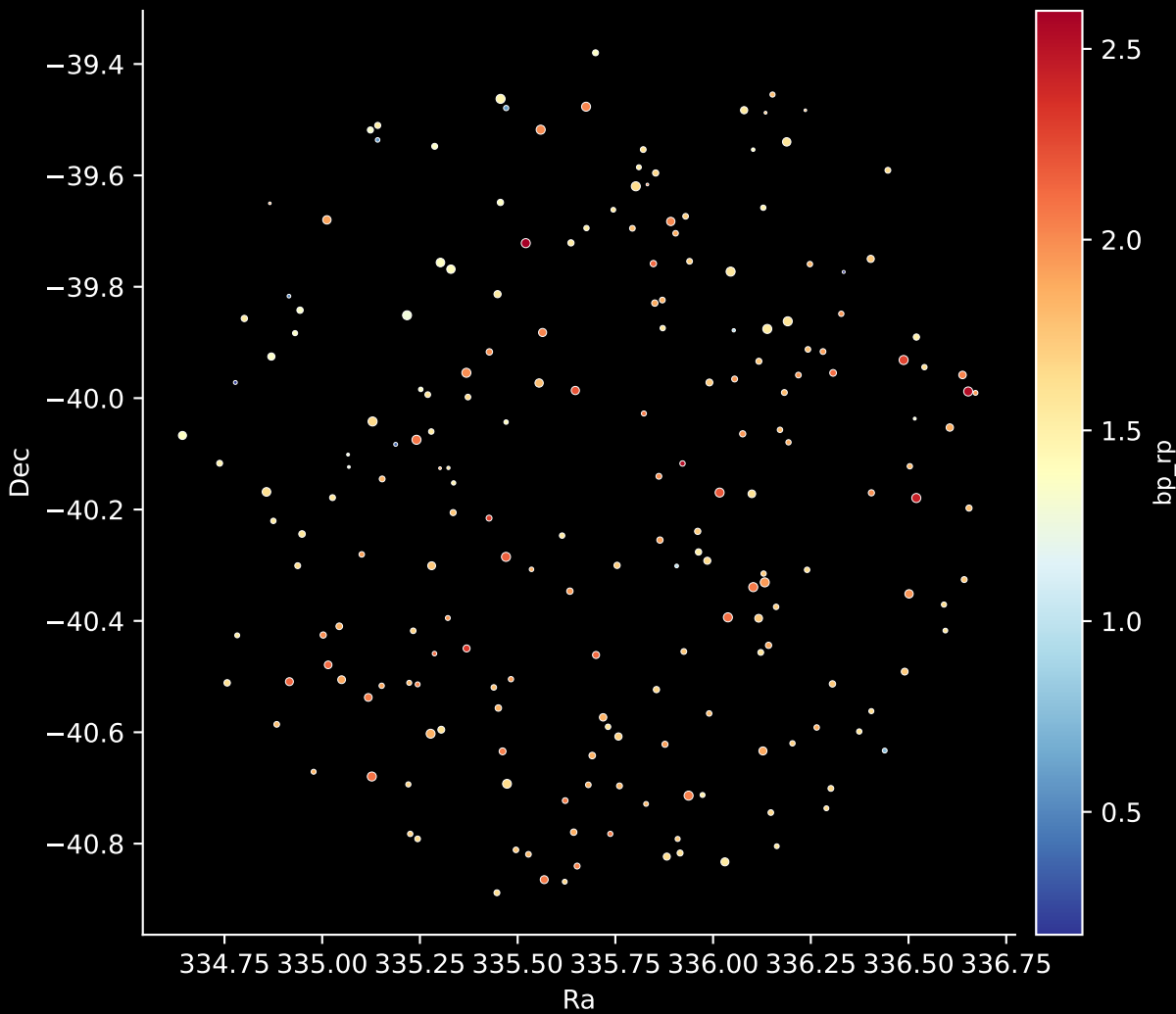
APOGEE DR17 Field: [335+12] Stars: 204
