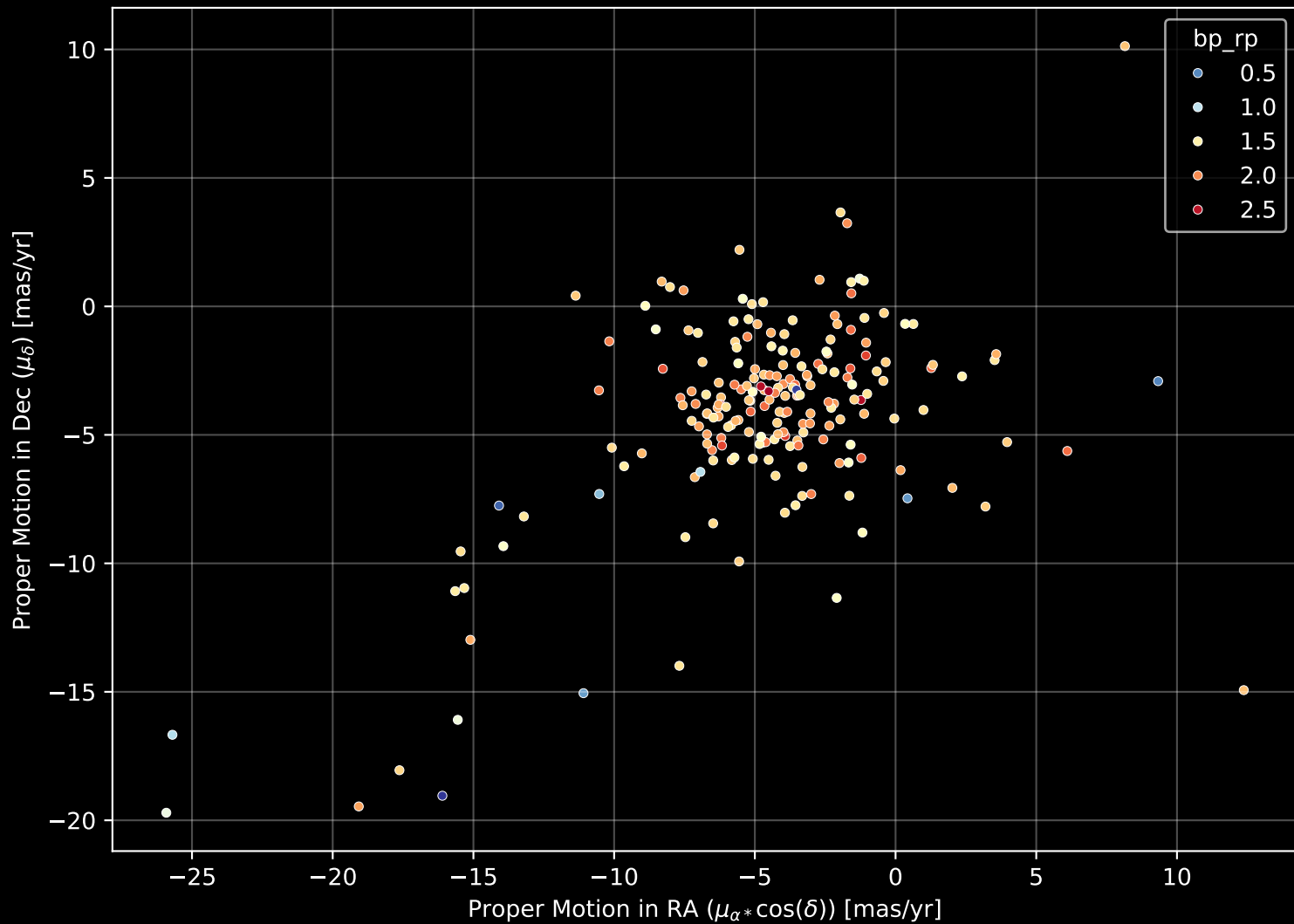
APOGEE DR17 Field: [335+12] Proper Motion Diagram (n= 204)
