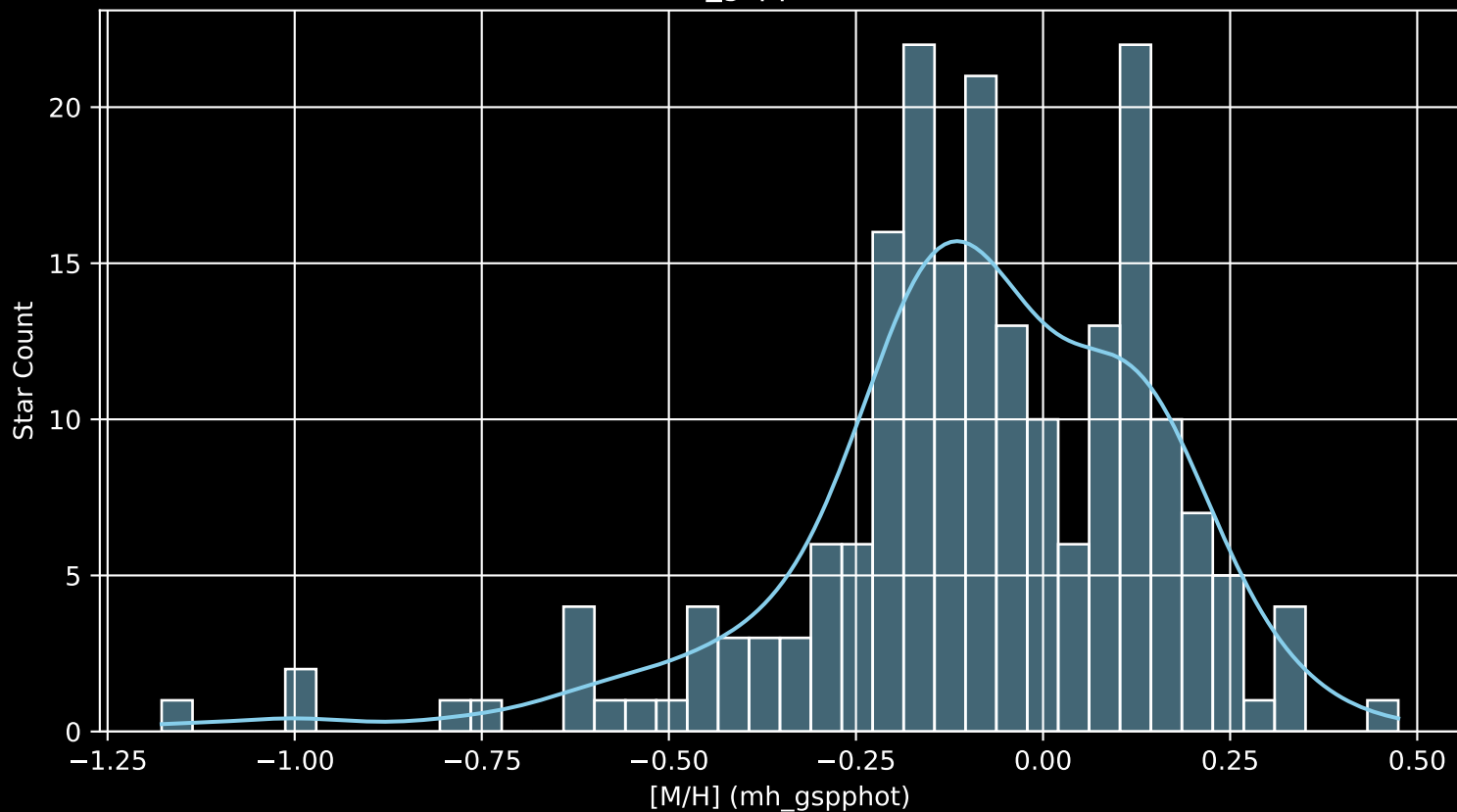
APOGEE DR17 Field: [335+12 [M/H] (mh_gspphot) (n= 203)
