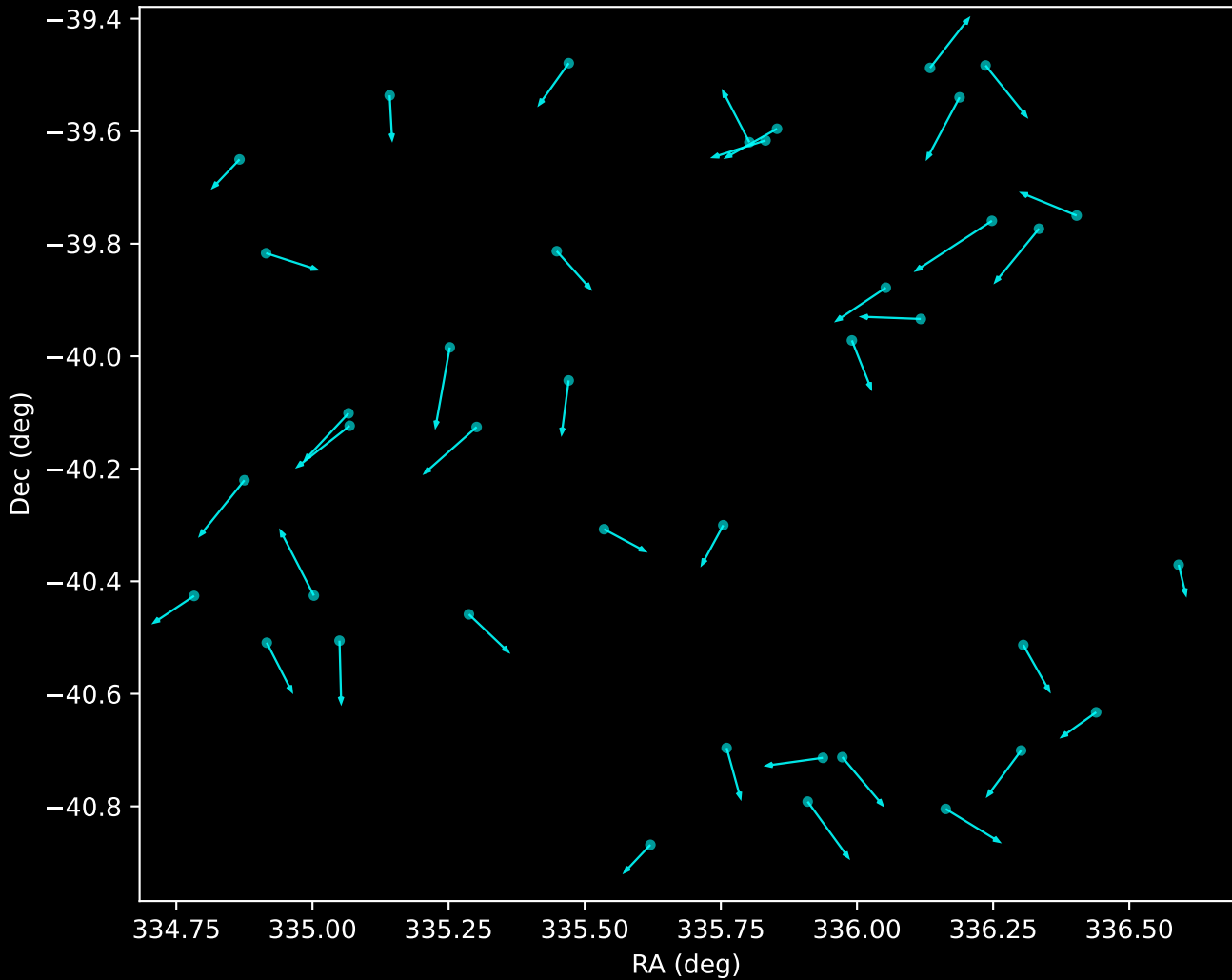
APOGEE DR17 Noise Stream Proper Motion Vectors (n=40)
