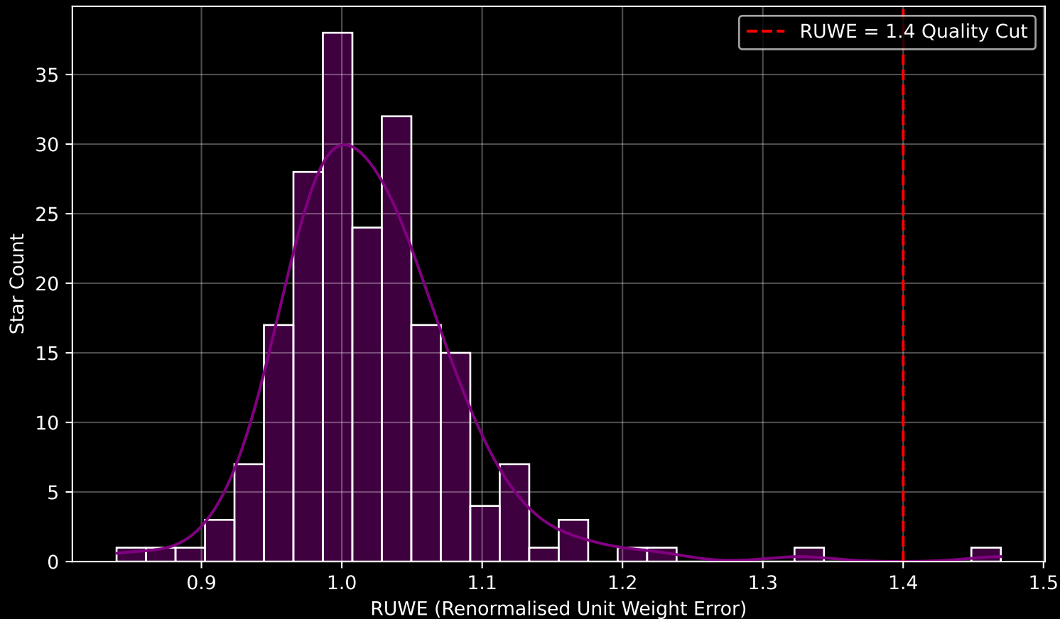
GAPOGEE DR17 Field [335+12] RUWE Distribution (n= 203)
