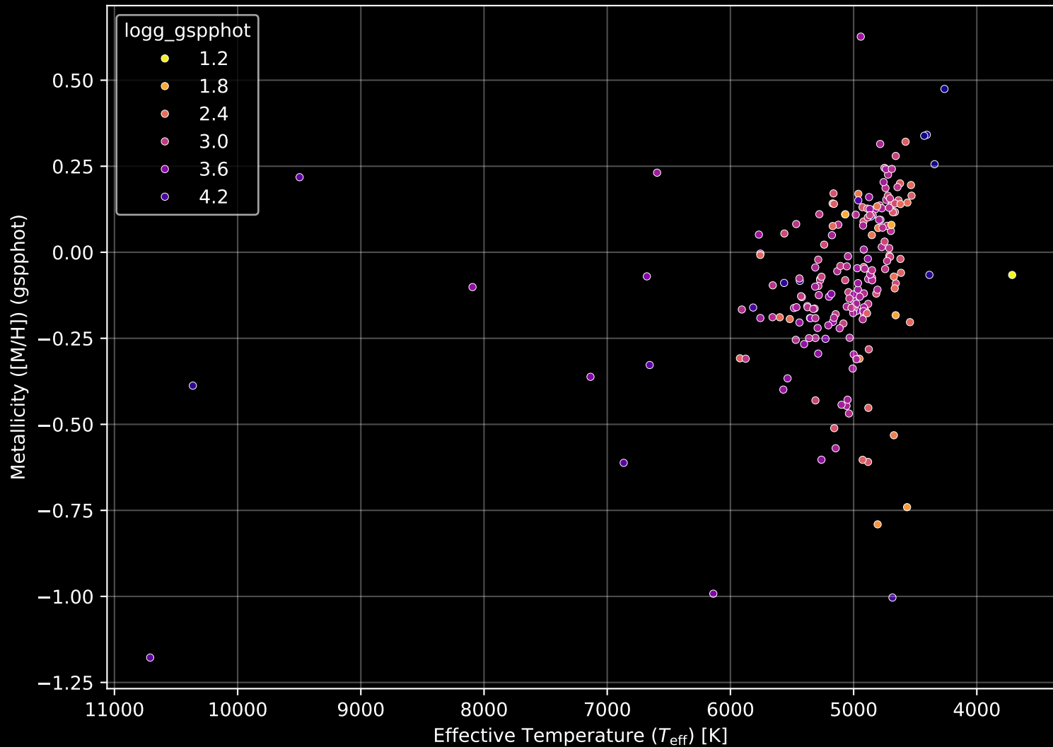
APOGEE DR17 Field: [335+12] Stellar Population Parameters (n= 204)
