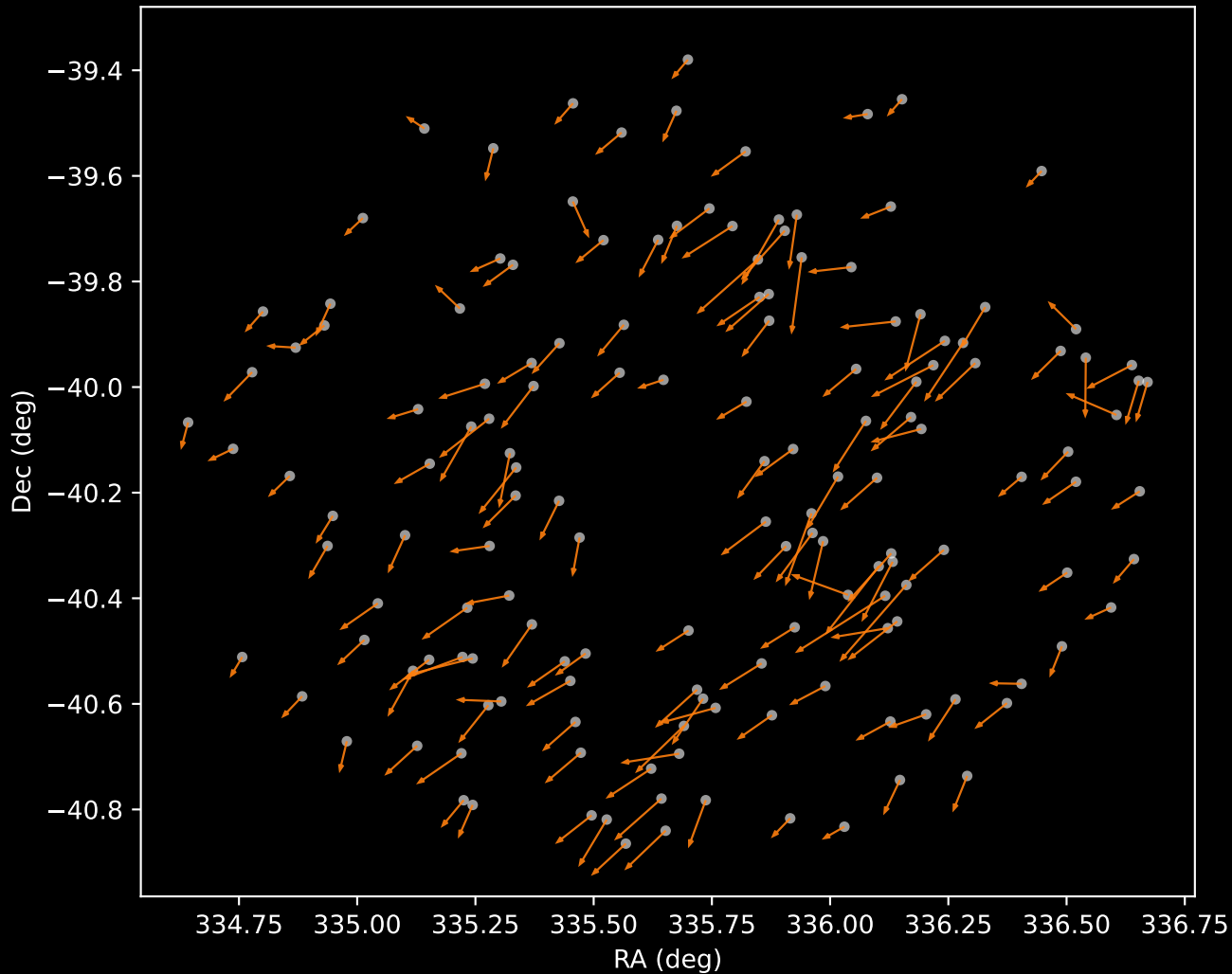
APOGEE DR17 Cluster 2 Proper Motion Vectors (n=153)
