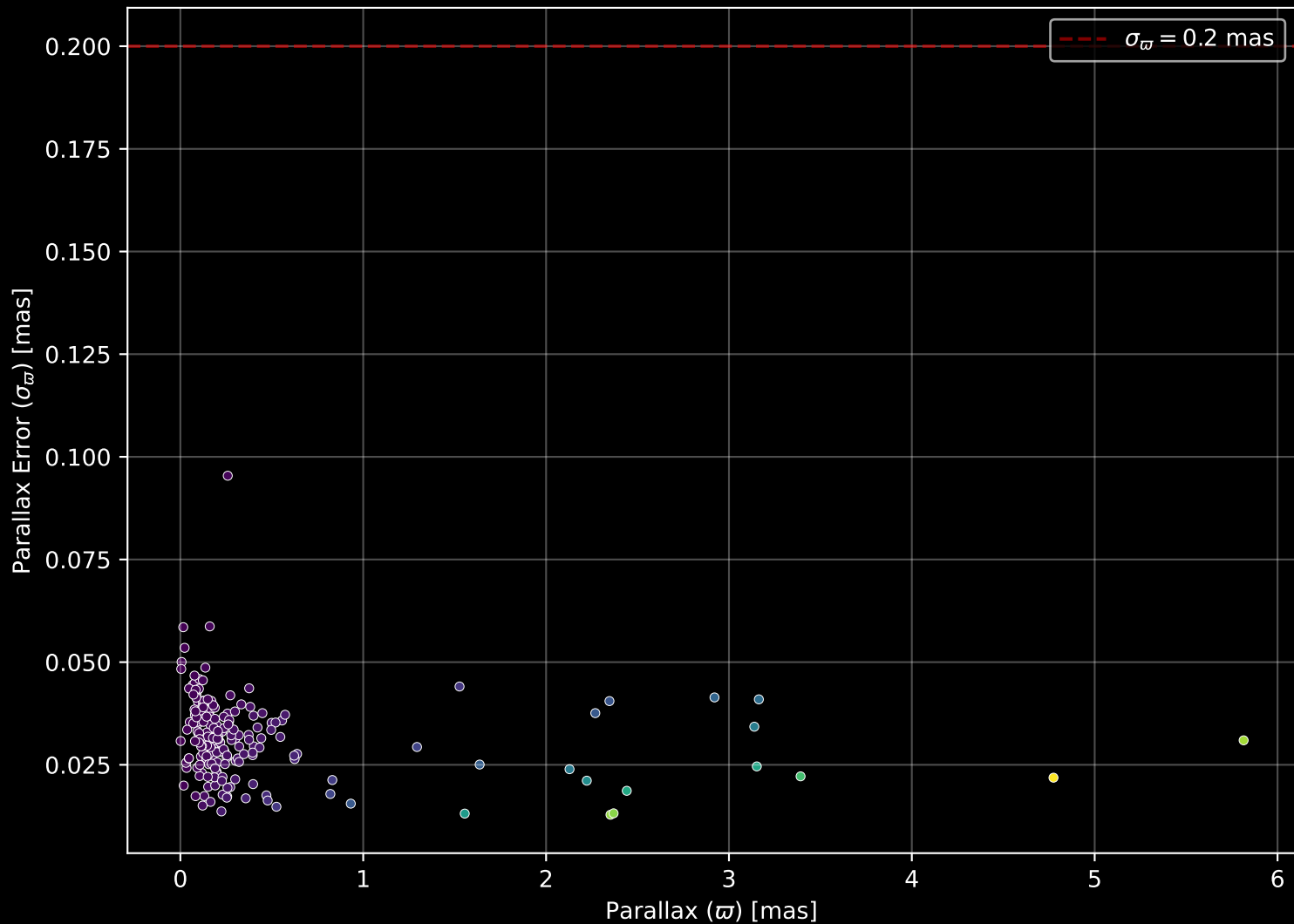
APOGEE DR17 Field: [335+12] Parallax Quality (n= 204)
