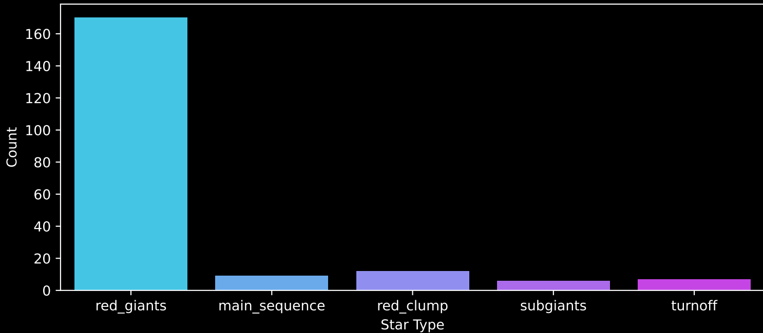
APOGEE DR17 Field: [335+12] Count plot of Star Type
